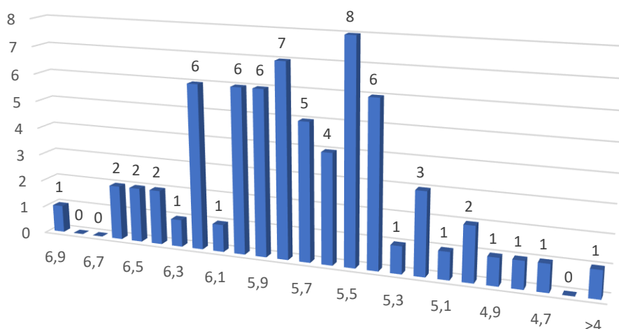
Detailed D-Score
